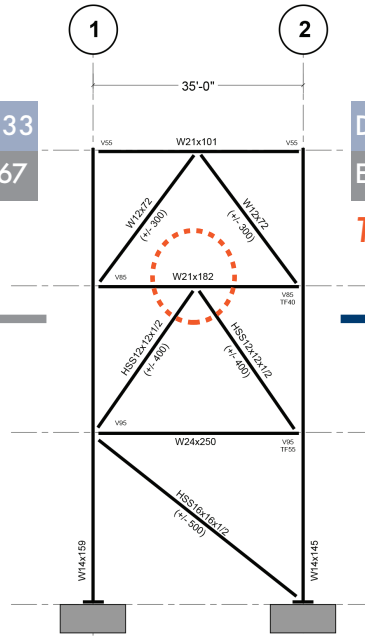
BF-1 ELEVATION ALONG GL A
